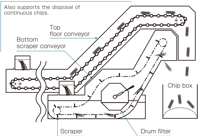
6 Coolant supply unit with take-up chip conveyor Chips collected in the center trough are transported outside of the machine by the chip conveyor. Two types of chip conveyors are provided to choose from depending on chip shape and material.
