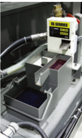
Oil skimmer
