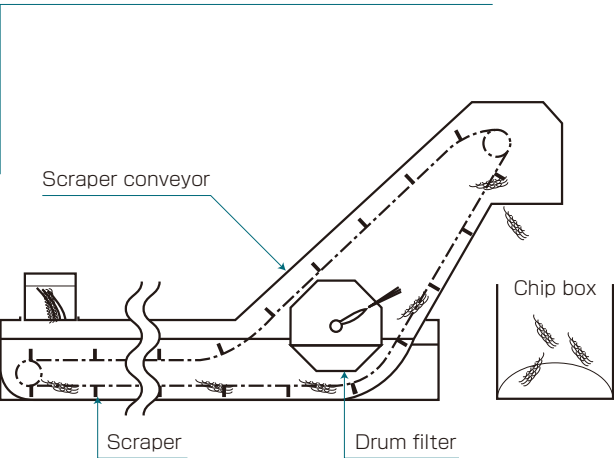
6 Coolant supply unit with take-up chip conveyor Chips collected in the center trough are transported outside of the machine by the chip conveyor. Two types of chip conveyors are provided to choose from depending on chip shape and material.
