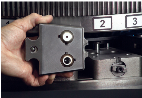
Quick-change die holders reduce set-up time to increase overall productivity.
