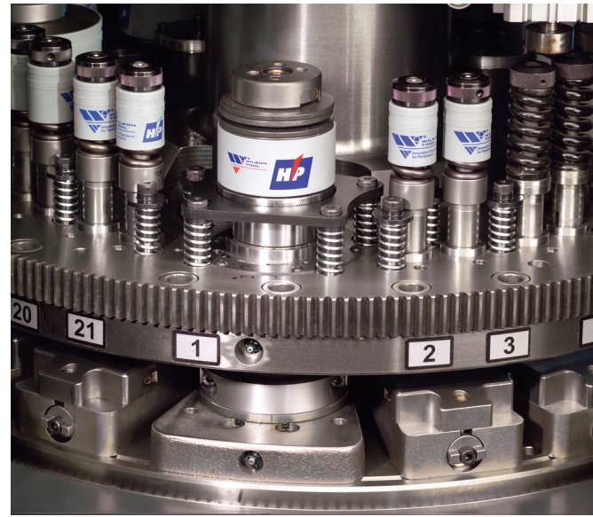
A 21-station turret configuration offers tremendous flexibility and capacity.
